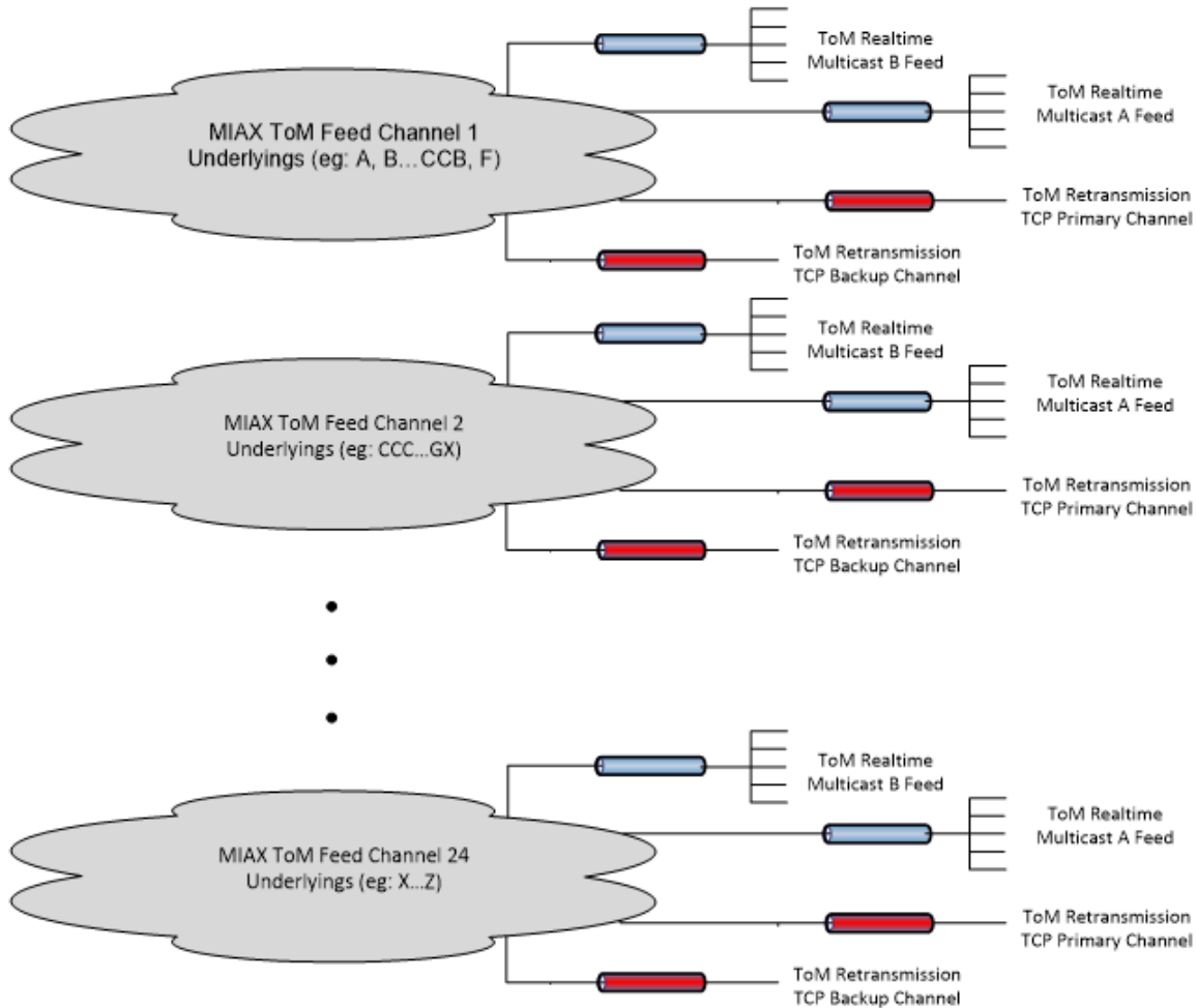
MIAX Top of Market (ToM) Architecture
